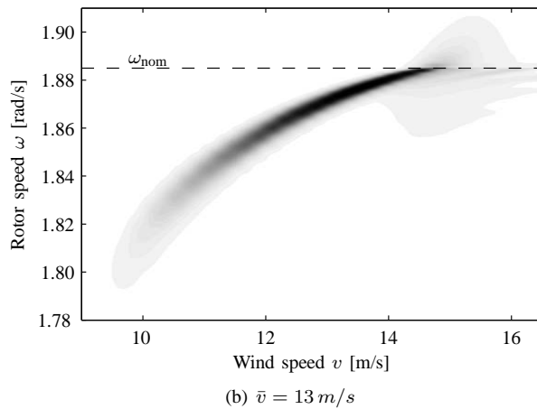
Fig. 4. Joint pdf of the rotor speed \omega(t) and the wind speed v(t) , obtained by marginalization over the pitch angle \theta(t) and the mode q(t) .
