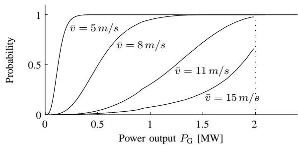
Fig. 6. Distribution function of the power output P_G , for several values of the mean wind speed \bar{v} . The discontinuity at P_G = P_{G,\text{nom}} for high wind speeds indicates that \mathbb{P}\{q(t) = B\} > 0 .
