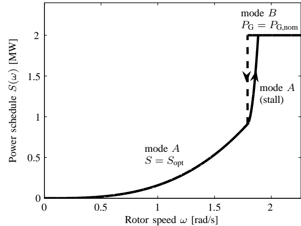
Fig. 2. Power schedule \omega \mapsto S(\omega)
